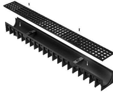
Rigola 100H70 + gratar fonta retea trafic 12.5 tone+Sistem de fixare 100x120x92
