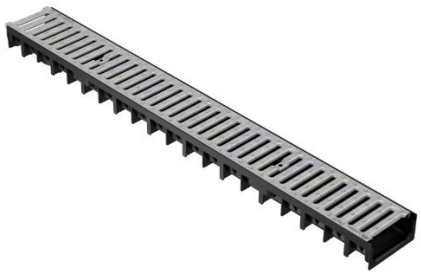
Rigola 100H30 + gratar otel zincat stantat trafic 1.5 tone 100x120x54,5
